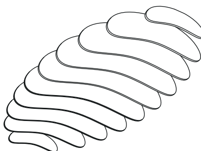
snow grains
